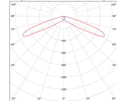
L2 cd - C180 — C90 - C270
