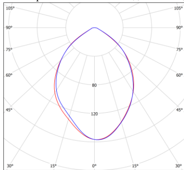
L1 cd - C180 — C90 - C270
