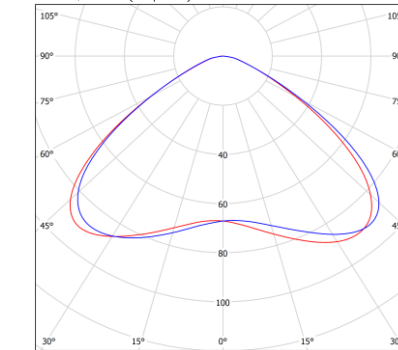
L3 cd - C180 — C90 - C270
