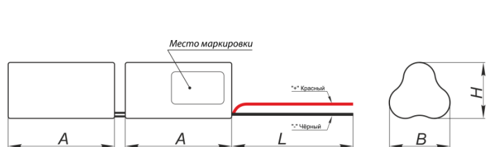
Батарея BS-3+3KRHT14/50-0.7/A-HB500-0-1 a27145
