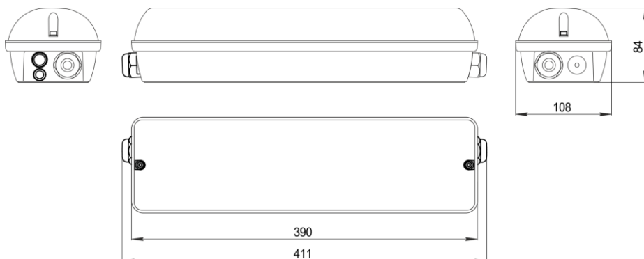
Рис.9 БАП BS-STABILAR2-81-B4-LED BOX IP65 (6,0-300 W / = 50-250 V)
