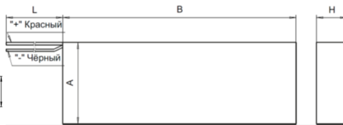
Рис.8 BS-10HRHT33/60-7.0/F-HB500-VHR-3N-1
