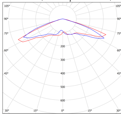
L2 cd/km C0 - C180 C90 - C270 η = 100%
